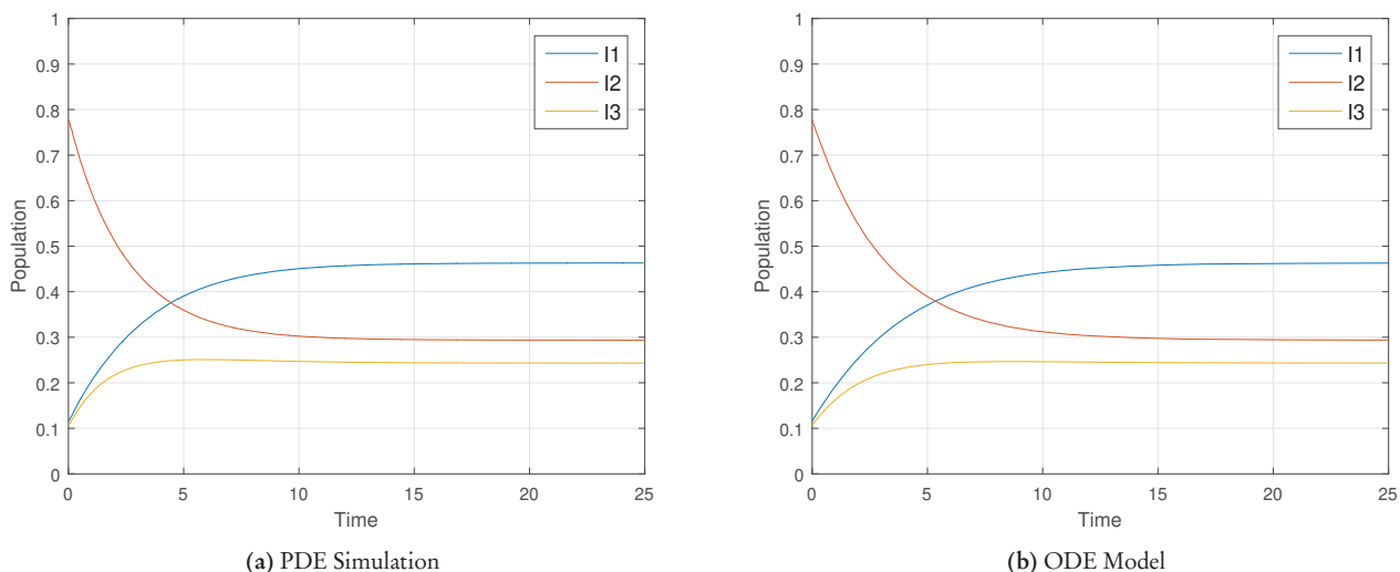
Figure 8. Comparison of the PDE and ODE response to a sudden change in fitness environment; D = 0.09
