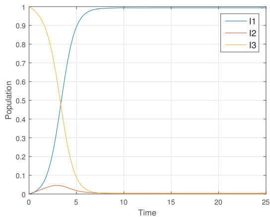
(f) ODE Model; D = 0.01
