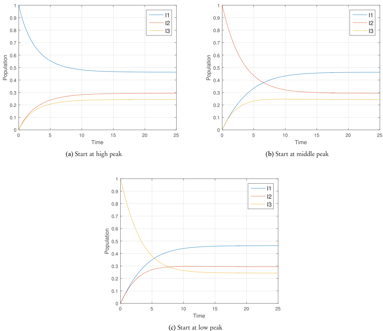
Figure 7. Results of the ODE model under the same parameters and three different initial conditions; D = 0.09
