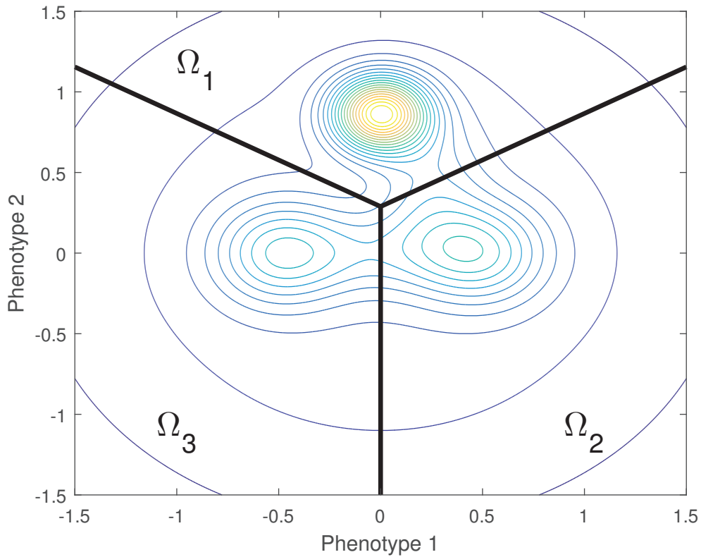
Figure 2. Partitioning the phenotype space into regions corresponding to network nodes. Contours show the fitness function peaks.
