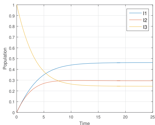
(b) ODE Model; D = 0.09
