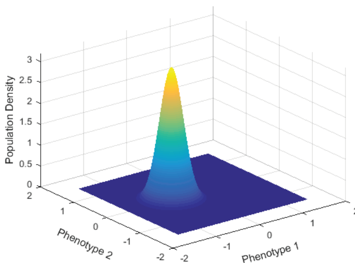
Figure 4. Starting population for transient simulations has 98% of the population in region 3
