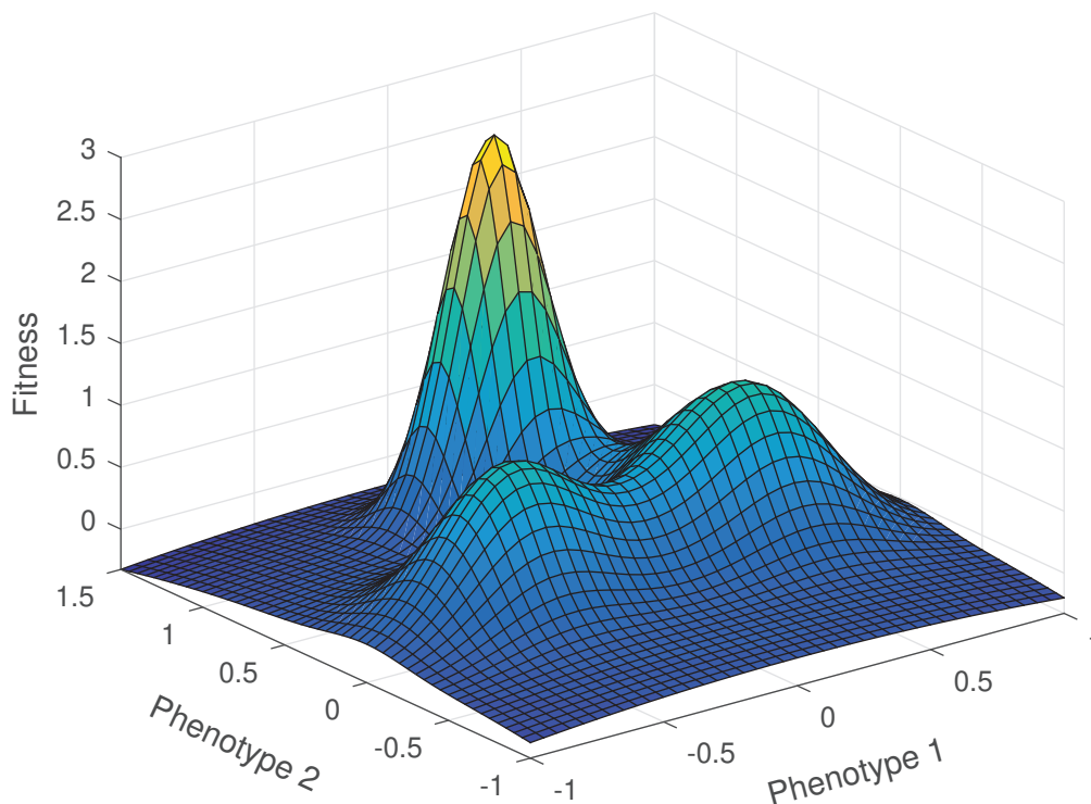
Figure 1. Fitness function used in the Fisher-Eigen equation
